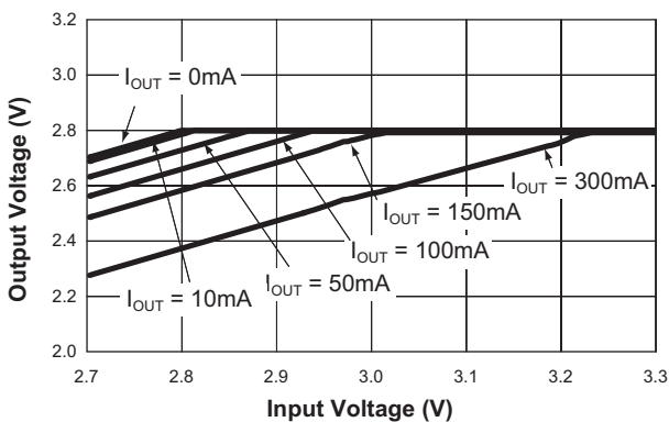
Dropout Characteristics
