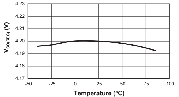
Constant Output Charge Voltage Regulation vs. Temperature (R SET = 8.06kΩ)
