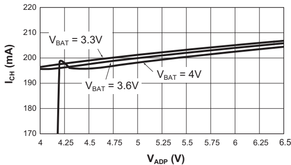
Constant Charging Current vs. Adapter Voltage (R SET = 8.06kΩ)
