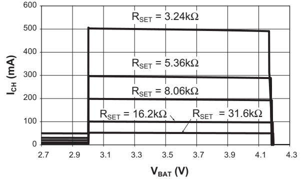
Charging Current vs. Battery Voltage (V ADP = 5V)
