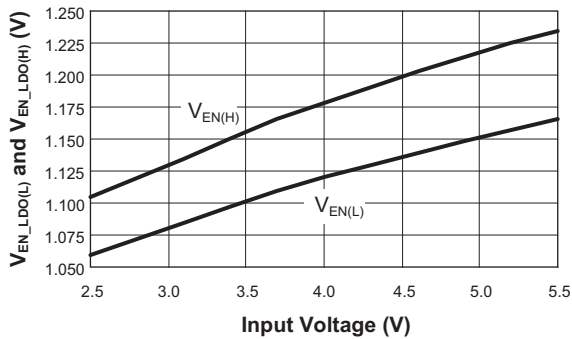
Enable Input High and Low Voltages vs. Input Voltage
